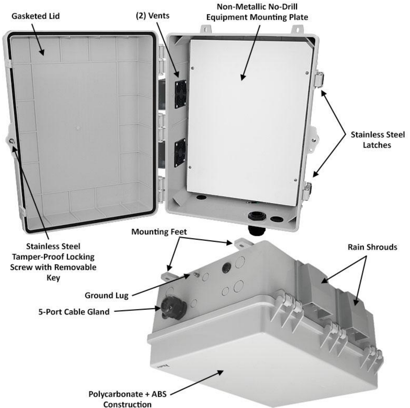
Model: NP171407CVM with Non-Metallic PVC Equipment Mounting Plate
