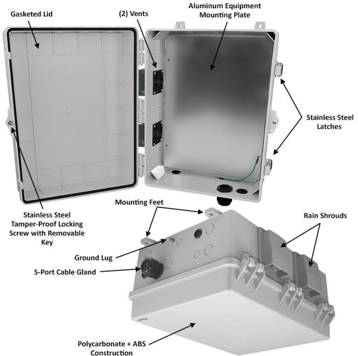
Model: NP171407CVP with Aluminum Equipment Mounting Plate
