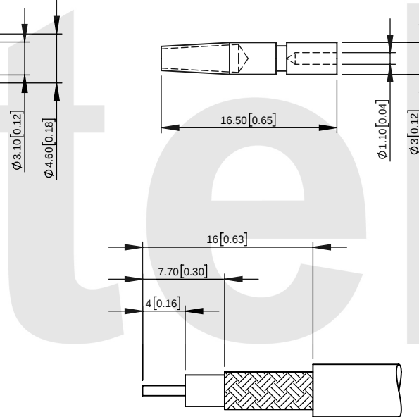
RECOMMENDED CABLE STRIPPING DIMENSIONS
