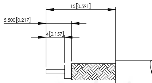
RECOMMENDED CABLE STRIPPING DIMENSIONS
