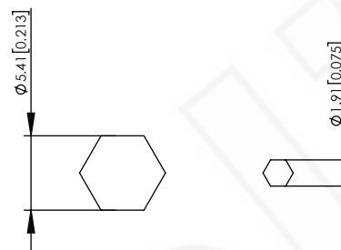
RECOMMENDED FERRULE AND PIN CRIMP SIZES
