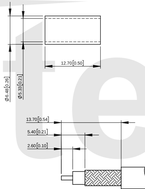
RECOMMENDED CABLE STRIPPING DIMENSIONS
