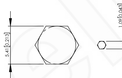
RECOMMENDED FERRULE AND PIN CRIMP SIZES
