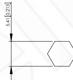
RECOMMENDED FERRULE CRIMP SIZE
