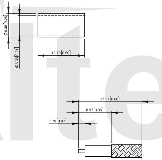
RECOMMENDED CABLE STRIPPING DIMENSIONS
