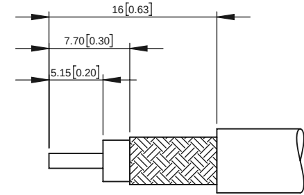
LMR400 RECOMMENDED CABLE STRIPPING DIMENSIONS
