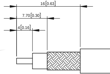
RG-8/X RECOMMENDED CABLE STRIPPING DIMENSIONS
