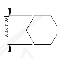
RECOMMENDED FERRULE CRIMP DIMENSIONS
