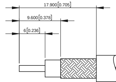
LMR400 RECOMMENDED CABLE STRIPPING DIM'S
