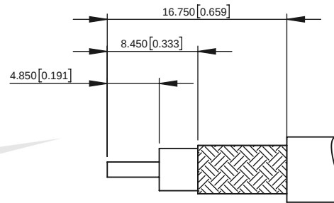
RG-8/X RECOMMENDED CABLE STRIPPING DIM'S
