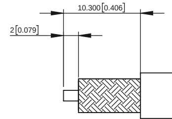
RECOMMENDED CABLE STRIPPING DIMENSIONS
