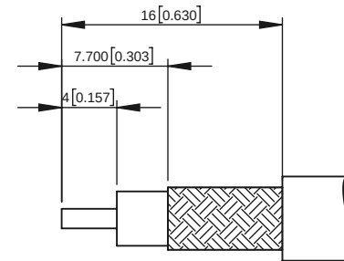
RECOMMENDED CABLE STRIPPING DIMENSIONS
