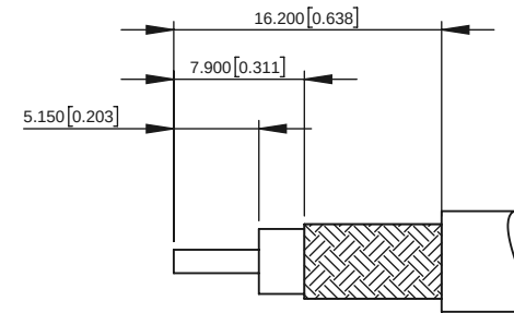
LMR240 RECOMMENDED CABLE STRIPPING DIMENSIONS
