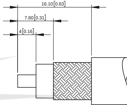
RECOMMENDED CABLE STRIPPING DIMENSIONS
