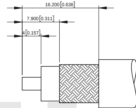
RECOMMENDED CABLE STRIPPING DIMENSIONS
