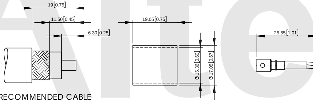
RECOMMENDED CABLE STRIPPING DIMENSIONS
