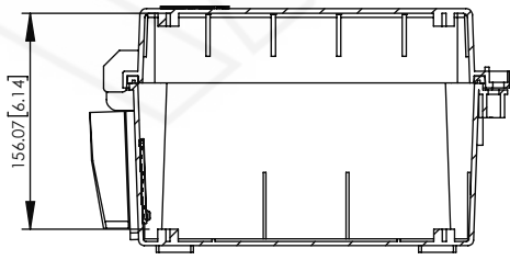
33, 26, AND 16mm CABLE KNOCKOUTS
