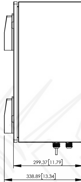
SECTION B-B
