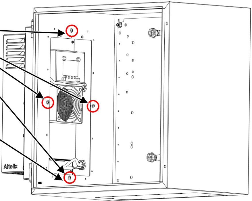
Screw with Rubber Bonded Washer
